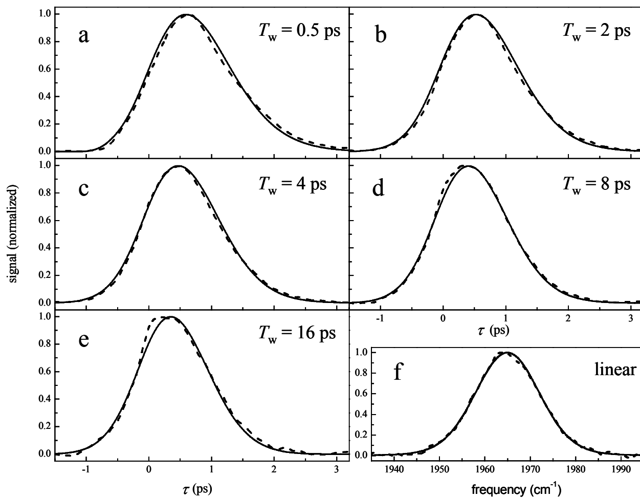
Figure S2. a) Experimental vibrational echo decay data at T_w = a) 0.5 ps, b) 2 ps, c) 4 ps, d) 8 ps, e) 16 ps, and f) linear spectrum for Ht -M61A/Q64N (dashed lines) overlaid with the best-fit vibrational echo decay and linear spectrum calculated from nonlinear response theory (solid lines) at 1965\text{ cm}^{-1} .
