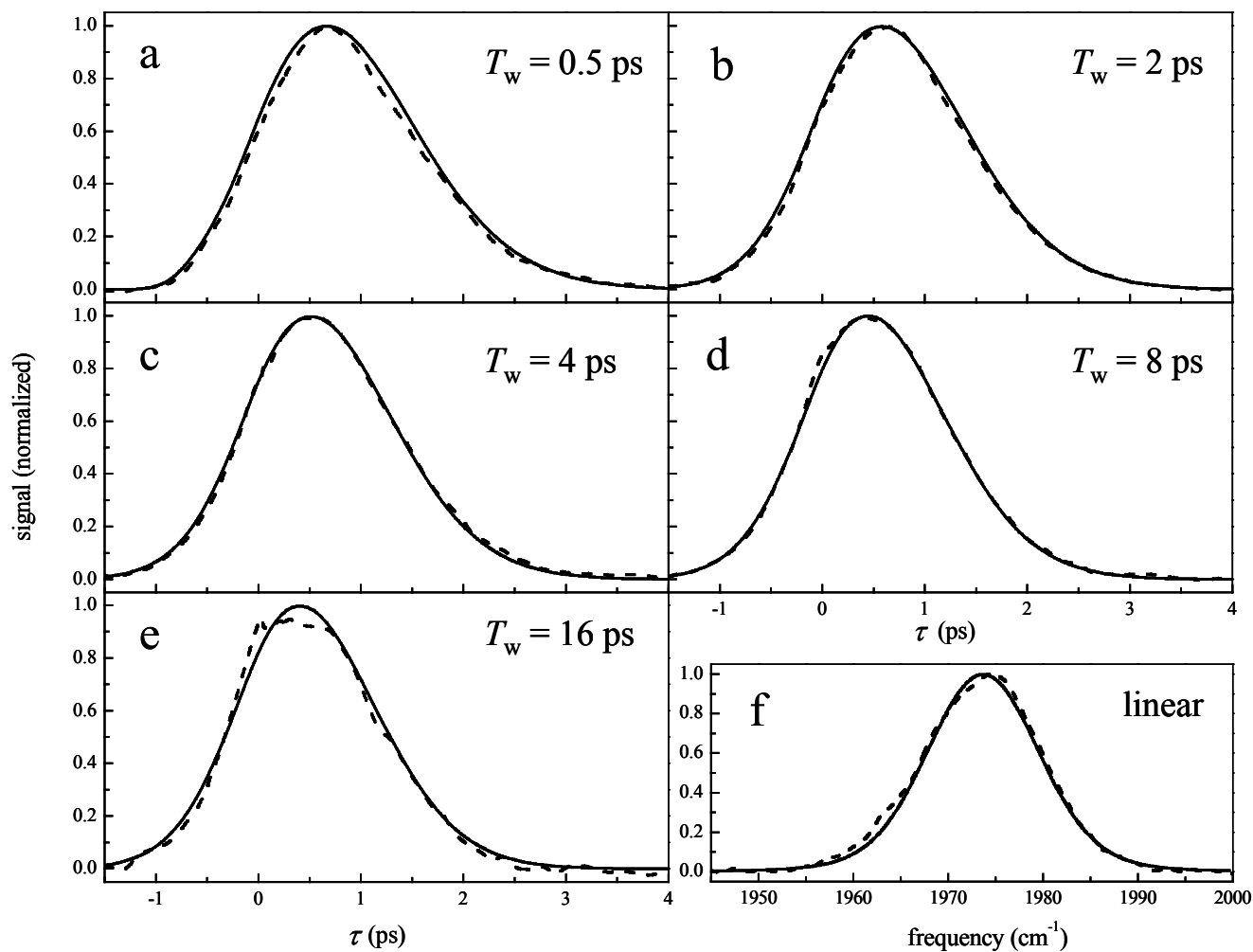
Figure S1. a) Experimental vibrational echo decay data at T_w = a) 0.5 ps, b) 2 ps, c) 4 ps, d) 8 ps, e) 16 ps, and f) linear spectrum for Ht -M61A (dashed lines) overlaid with the best-fit vibrational echo decay and linear spectrum calculated from nonlinear response theory (solid lines) at 1975 cm -1 .
